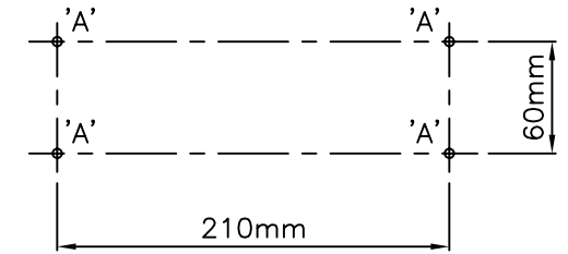
DRILLING DETAIL
