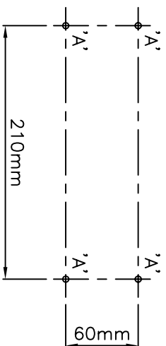
DRILLING DETAIL
