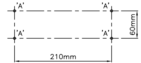
DRILLING DETAIL
