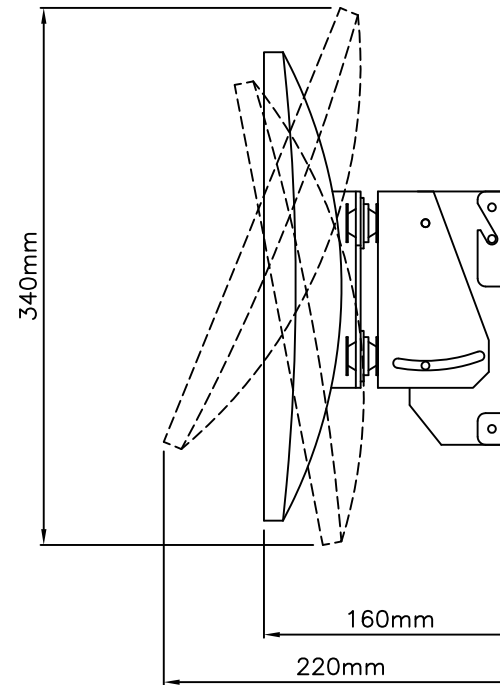
WALL MOUNTING DETAIL
