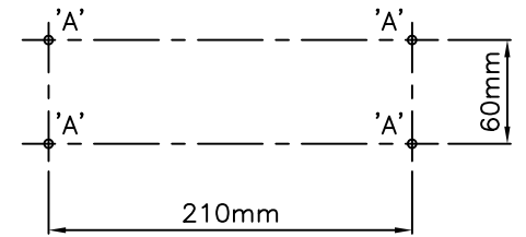
DRILLING DETAIL
