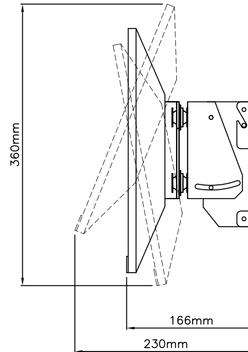
WALL MOUNTING DETAIL
