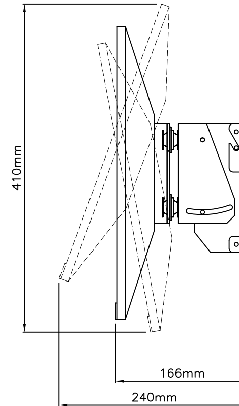
WALL MOUNTING DETAIL
