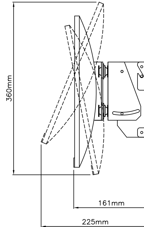
WALL MOUNTING DETAIL
