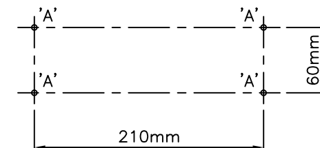
DRILLING DETAIL
