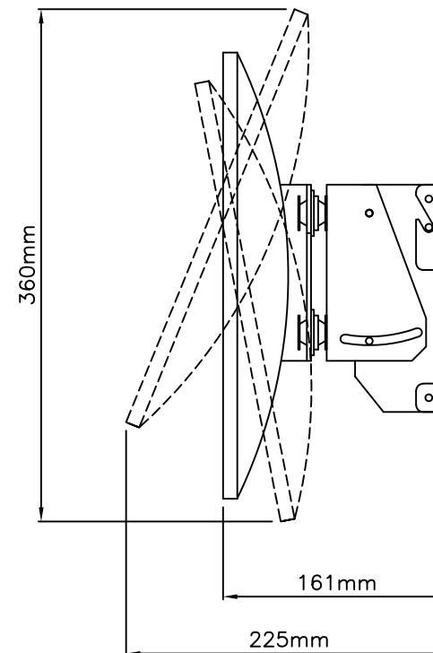
WALL MOUNTING DETAIL
