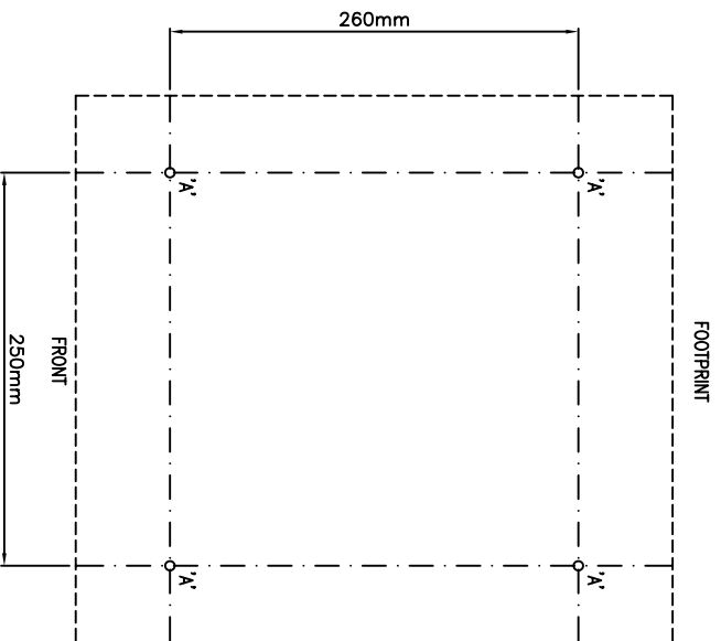
DRILLING DETAIL
