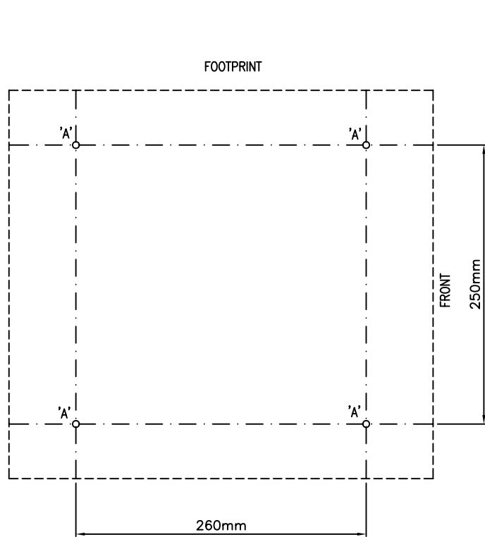
DRILLING DETAIL
