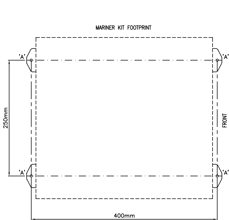
STUD LOCATION DETAIL WHEN UTILISING CB100 BRACKETS
