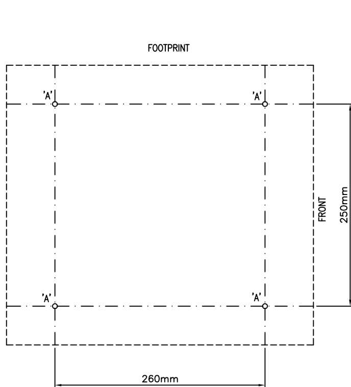
DRILLING DETAIL
