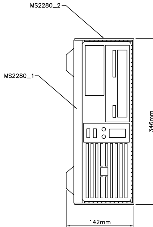
FRONT ELEVATION
