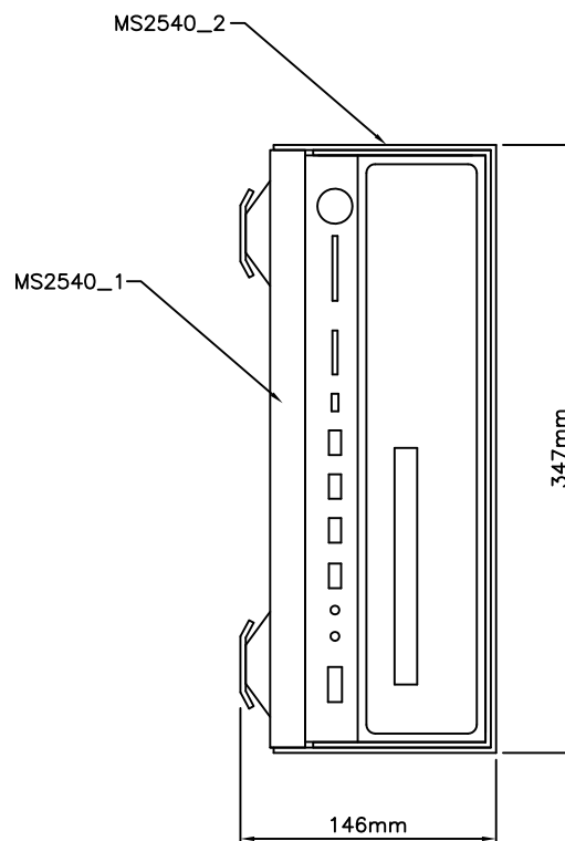
FRONT ELEVATION
