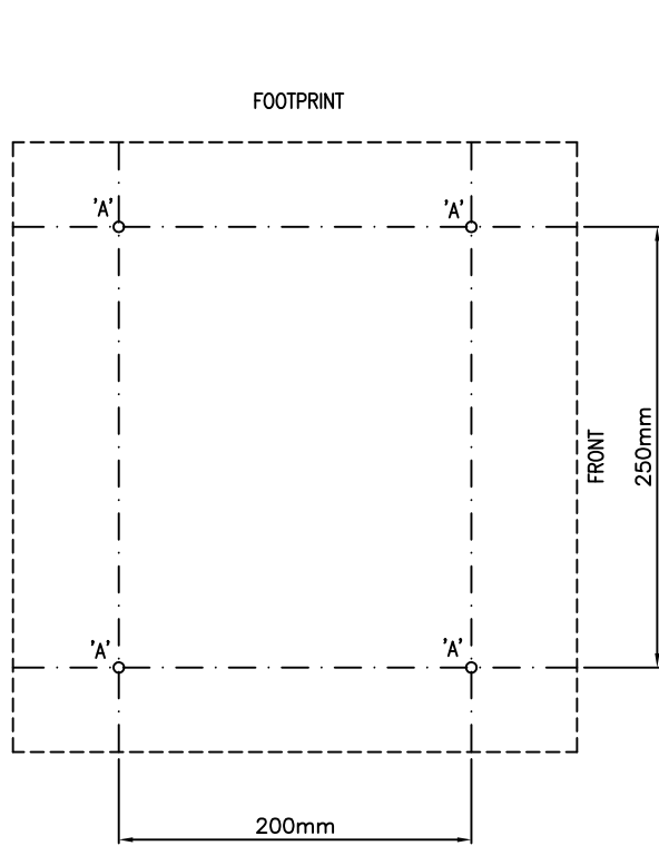
DRILLING DETAIL
