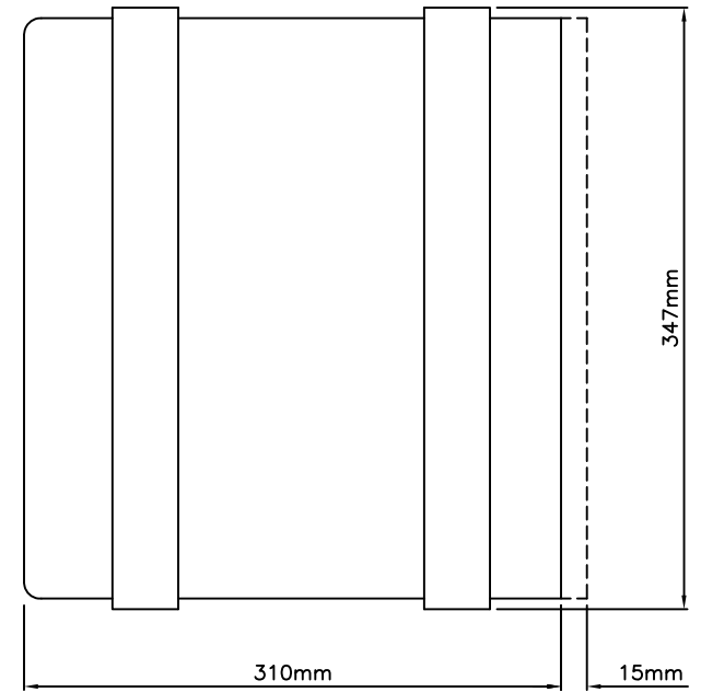
SIDE ELEVATION
