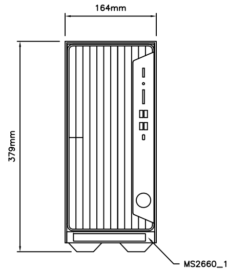
FRONT ELEVATION
