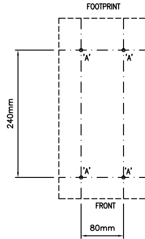
DRILLING DETAIL
