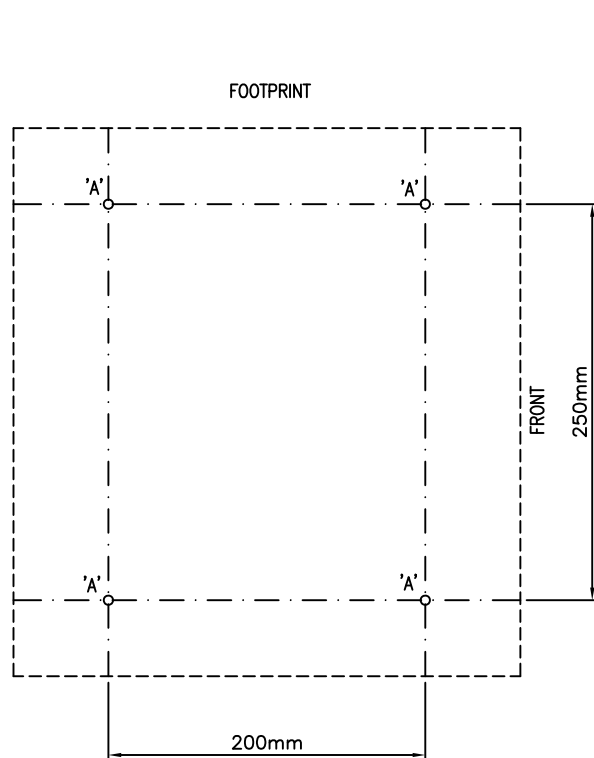
DRILLING DETAIL
