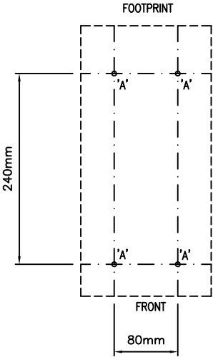
DRILLING DETAIL
