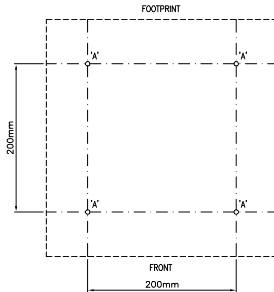
DRILLING DETAIL
