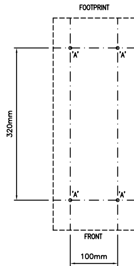
DRILLING DETAIL
