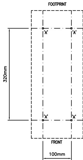
DRILLING DETAIL
