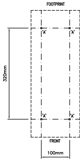
DRILLING DETAIL
