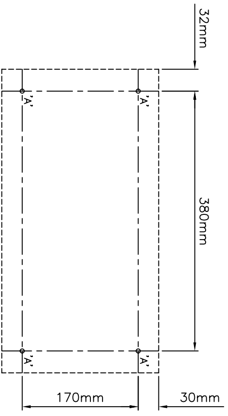
DRILLING DETAIL
