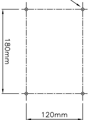
WALL MOUNTING DETAIL
